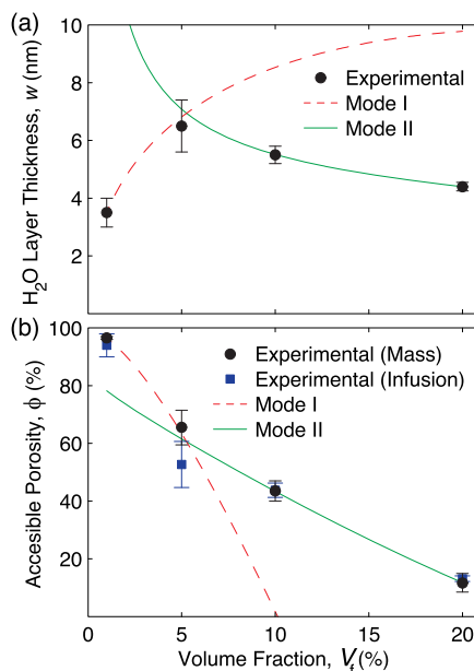
Figure 3. (a) Water layer thickness ( w ) as a function of CNT volume fraction ( V_f ) showing the nonlinear and non-monotonic dependence of the physisorption process on CNT proximity and indicating a change of mechanism at V_f \sim 5.3\% . (b) Plot of the accessible porosity of the CNT arrays evaluated using the ratio of the dry and wet CNT array mass (see eq 2 and Table S3 in the Supporting Information) and infusion of the CNT arrays with a hydrophobic phenolic resin. The plot illustrates the strong influence of the thickness of the physisorbed water layer, especially at V_f \geq 5\% .
