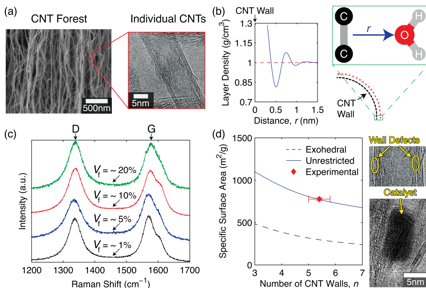
Figure 1. (a) HRSEM image showing the morphology of an as-grown CNT forest and HRTEM image showing the structure of individual CNTs that make up the forest. (b) Plot of the layer density profile of water physisorbed onto the surface of a CNT from a previously reported MD simulation illustrating the strong influence of film thickness for thin ( \leq 1 nm) films of physisorbed water. 21 (c) Raman spectra illustrating that the CNTs used in this study had a significant number of defects ( I_G/I_D ratios \leq 1 ). (d) Plot of the specific surface area as a function of number of CNT walls for CNTs with no wall defects (exohedral adsorption) and with wall defects (unrestricted adsorption), and HRTEM images showing that the multiwalled CNTs used here are capped and have a significant number of wall defects.
