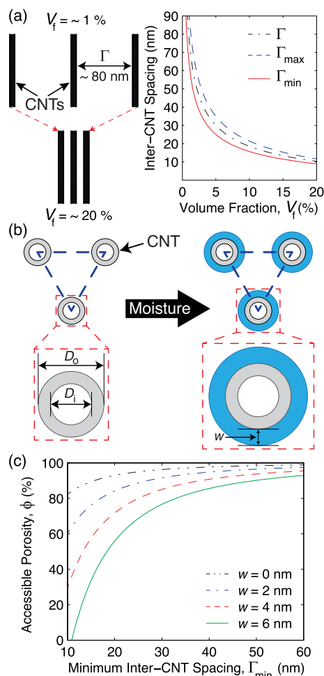
Figure 2. (a) Geometry and results of the inter-CNT spacing analysis performed using a previously reported continuous coordination model. 55 (b) Geometry used to model the exohedral layer-like physisorption of water molecules on the CNTs in the forests. (c) Plot of the available porosity as a function of minimum inter-CNT spacing for water layers up to 6 nm thick.
